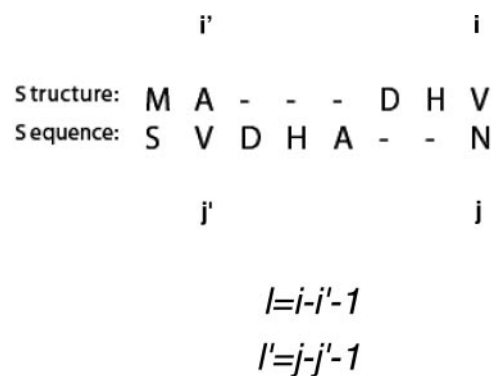
Fig. 1. Definition of a gap. i, i' and j, j' are residue positions on the structure and sequence, respectively. A single gap can include deletions and insertions on either the sequence or structure and is defined by all four indices i, i', j and j' .
