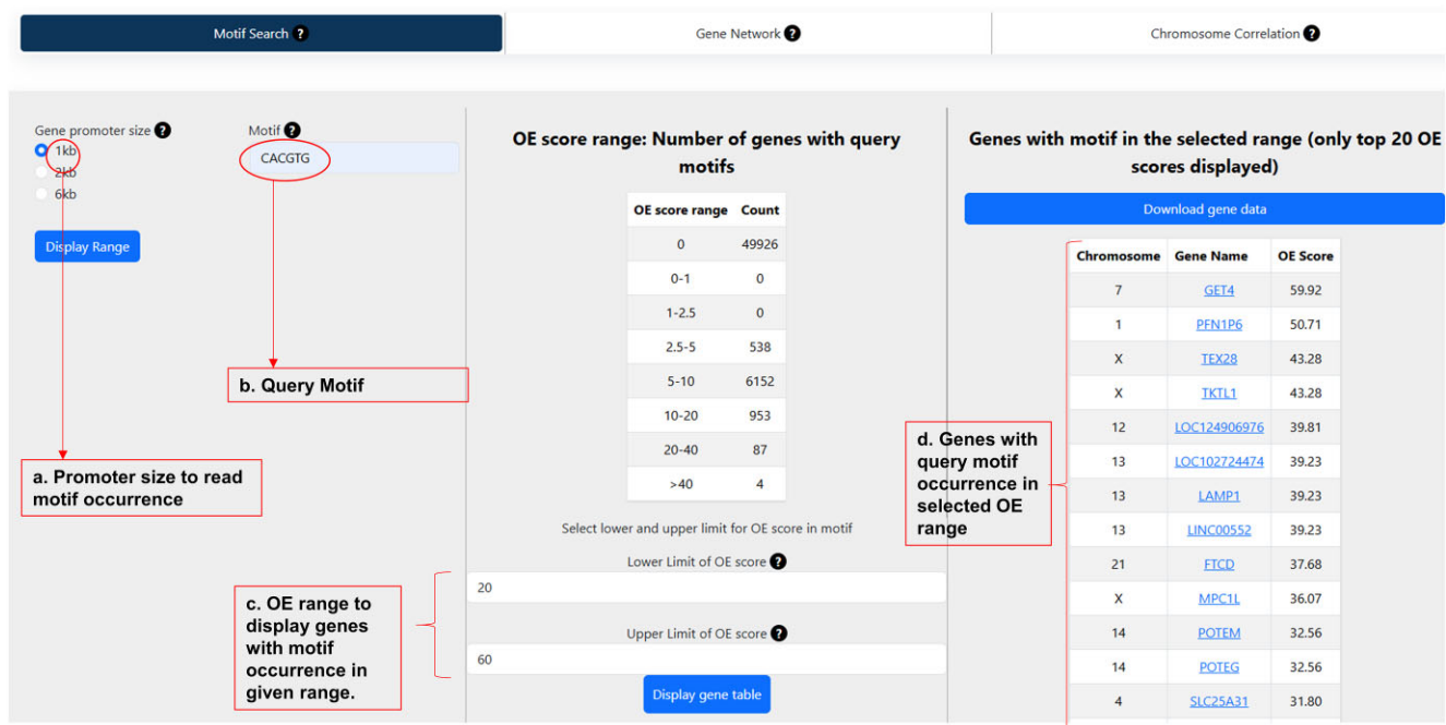
Figure 1. The description of 'Motif search' option on MAGNETIC. The text boxes labeled a–d explain the different parameters of the query search and the output results.
