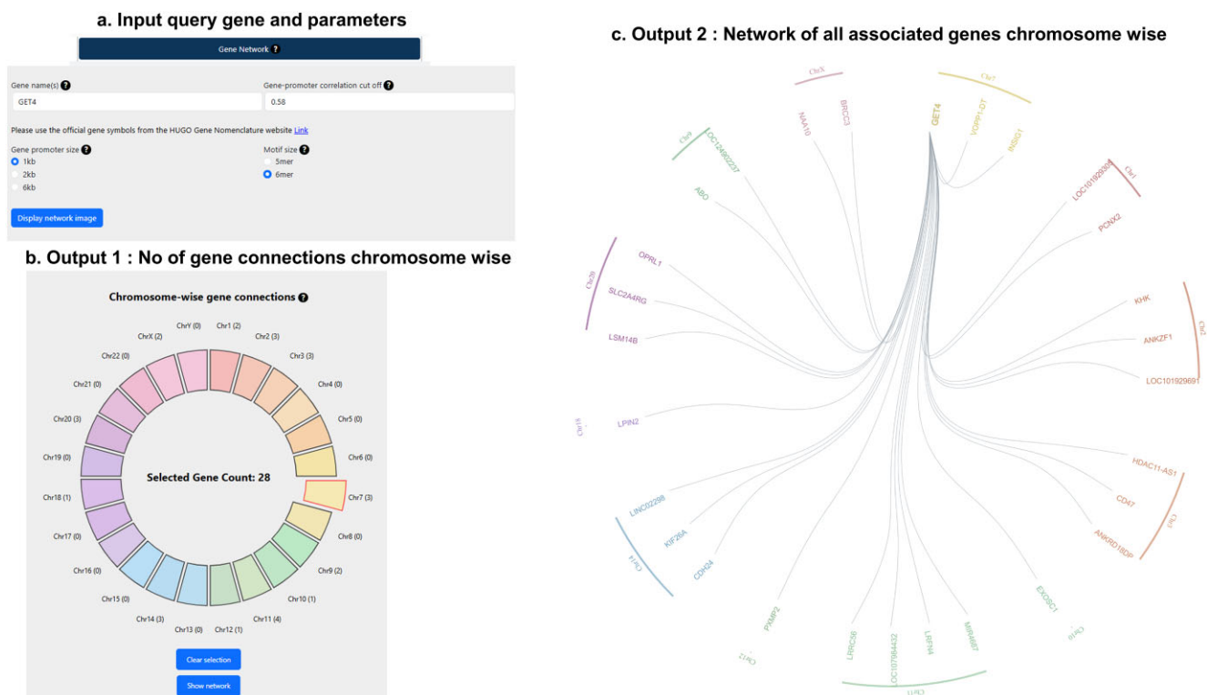
Figure 2. Using the 'Gene network' option of MAGNETIC for a single query gene. (A) The input query gene, 'GET4', and parameters of motif size, promoter size, and correlation cut-off. (B) The first output displays the gene associations per chromosome above the input correlation cut-off threshold. The chromosome housing the query gene is highlighted with a red border. (C) The second part of the output shows the gene regulatory network of associations with the query gene. The different gene colours represent the different chromosomal locations of the associated genes.
